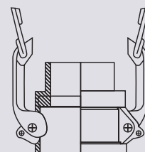
Female/hosetail for welding
