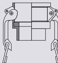
Male/BSP/Female
