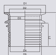
Tri-clamp Coupling With Hose Tail
