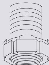
Female with Serrated Hose Tail
