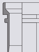
Male Couling With Hose TailHembra
