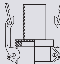
With hositail female
