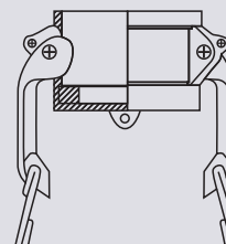
Female dustcap
