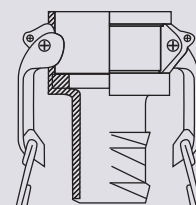
Female for CX Hose
