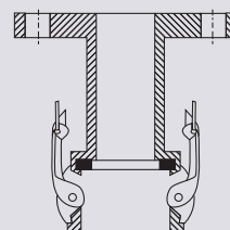
Flange coupler
