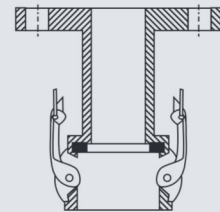
Flange coupler
