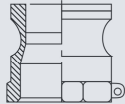
Male/BSP/Female
